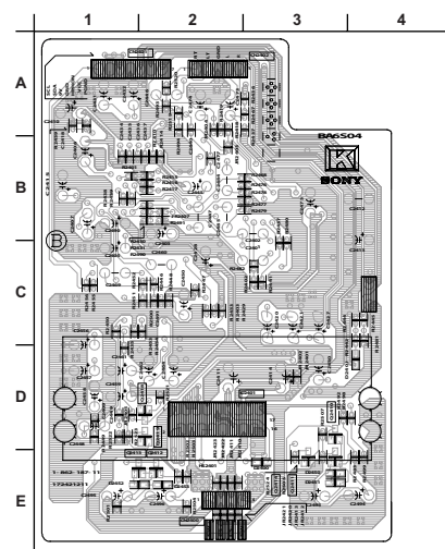
CONDUCTOR SIDE (KV-21FA310 ONLY)
