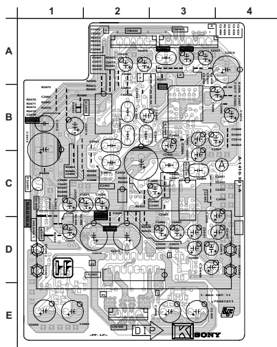
COMPONENT SIDE (KV-21FA310 ONLY)
