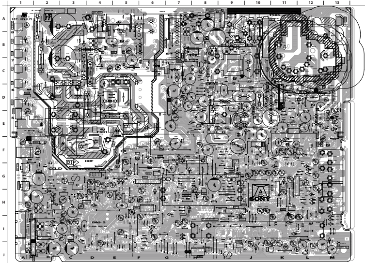
A BOARD LOCATOR LIST CONDUCTOR SIDE
